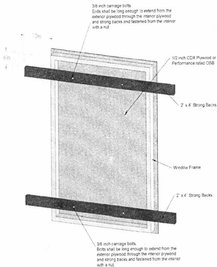
FIGURE A103.1(1) BOARDING OF DOOR OR WINDOW
