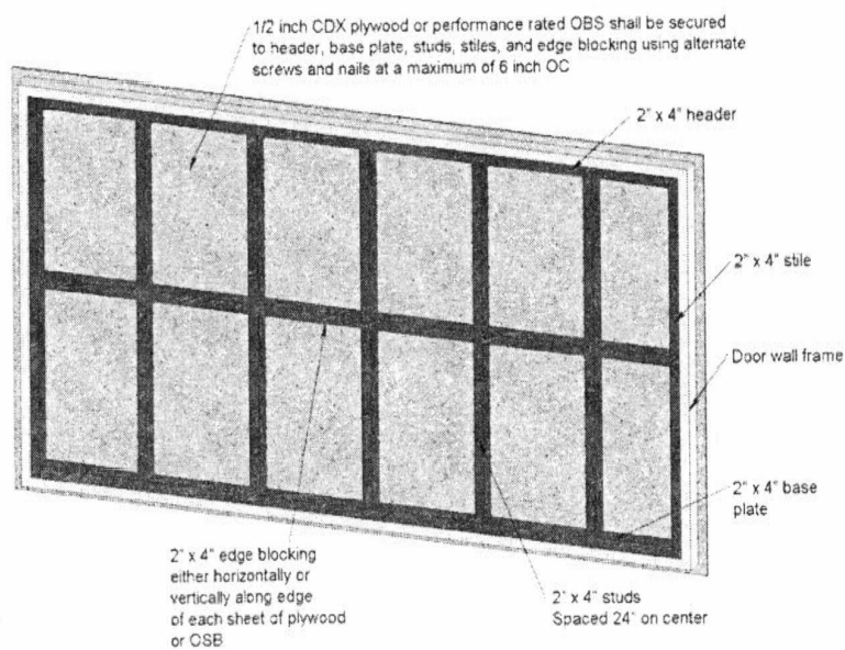
FIGURE A103.1(2) BOARDING OF DOOR WALL
